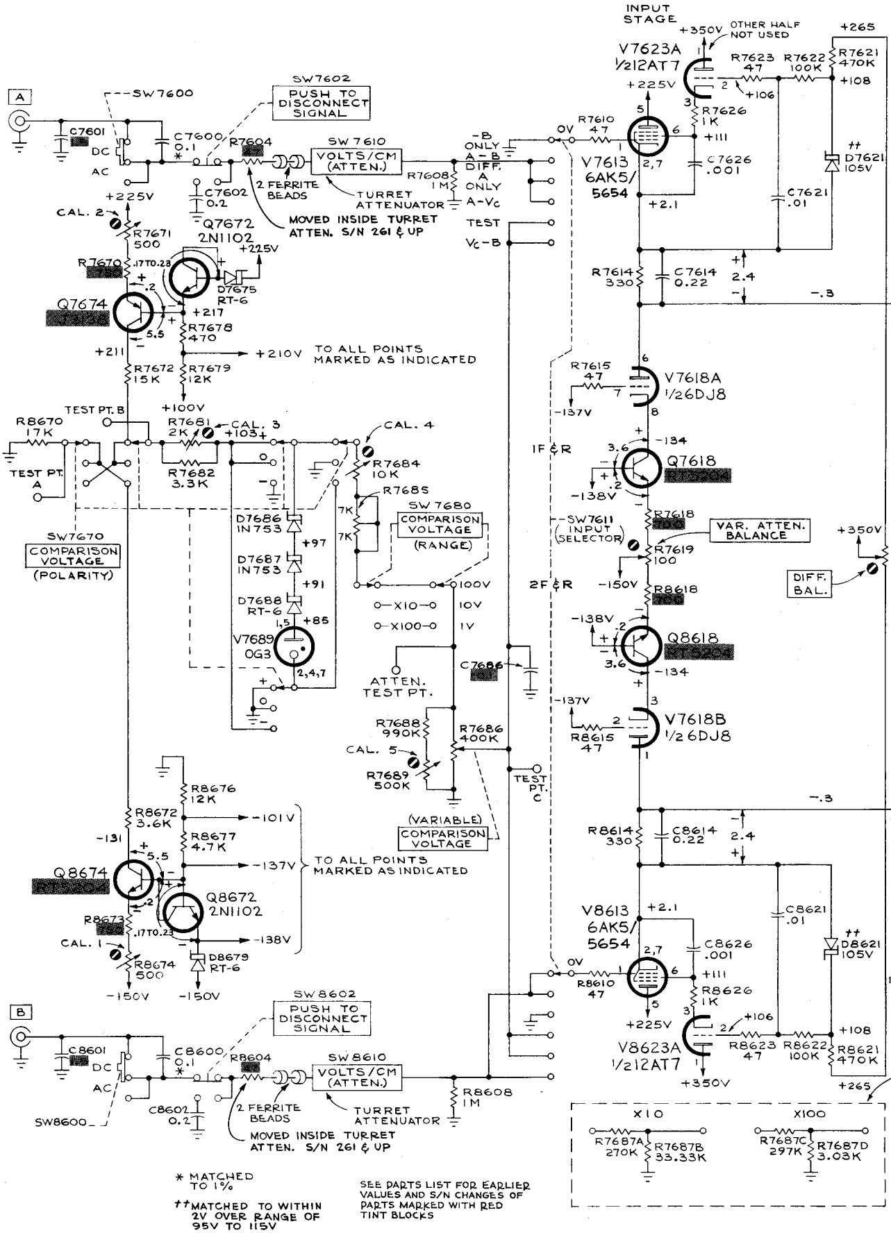
TYPE Z PLUG-IN UNIT
