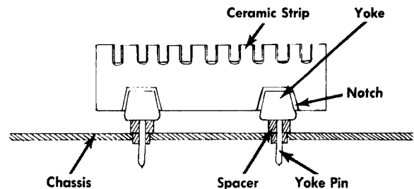
Fig. 4-2. Installation of ceramic terminal strips.
