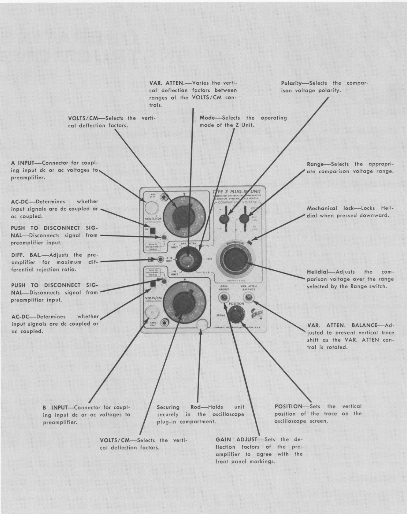
Fig. 2-1. Functions of front-panel controls, input connectors, Securing Rod, and Mechanical Lock.
